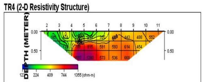
Figure 2d: 2-D Resistivity image tr4
