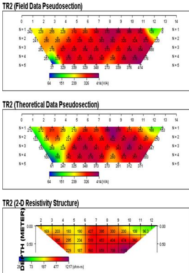
Figure 3b: Kaolinated 2-D resistivity image
