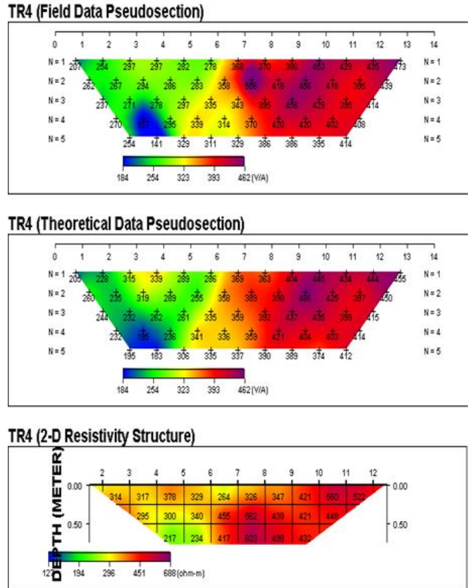
Figure 3d: Kaolinated 2-D Resistivity image
