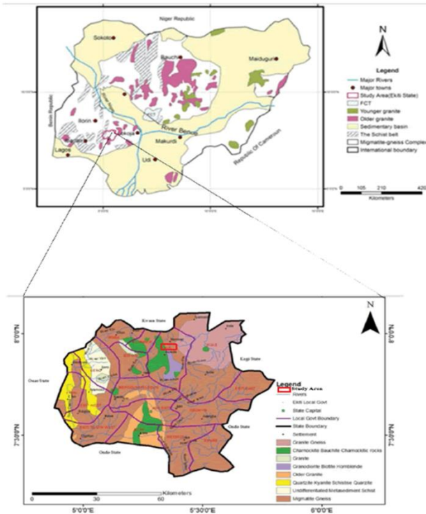
Figure 1: Geological map showing minerals deposit over parts of the study area (Oke, 2023).
