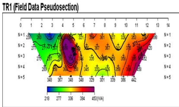
Figure 2a: 2-D Resistivity image at tr1
