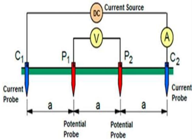
Figure 2: Diagram showing the pole configuration {7}.
